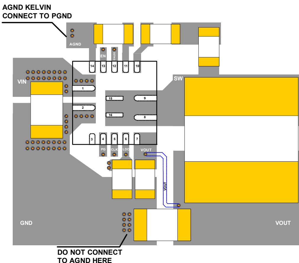
Figure 9—Recommend Layout
